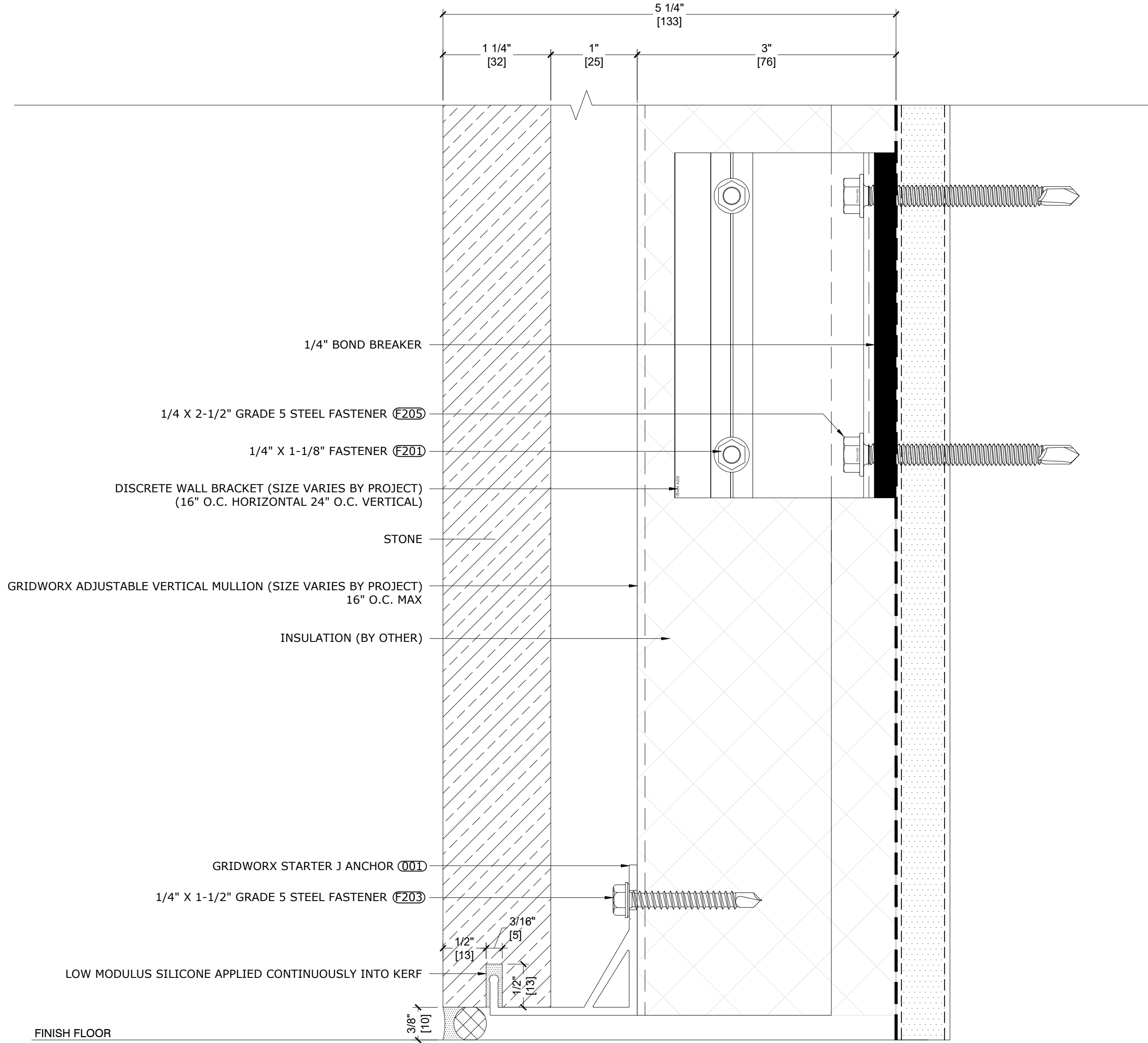
3 SECTION DETAIL - STARTER REF: ST2.01
