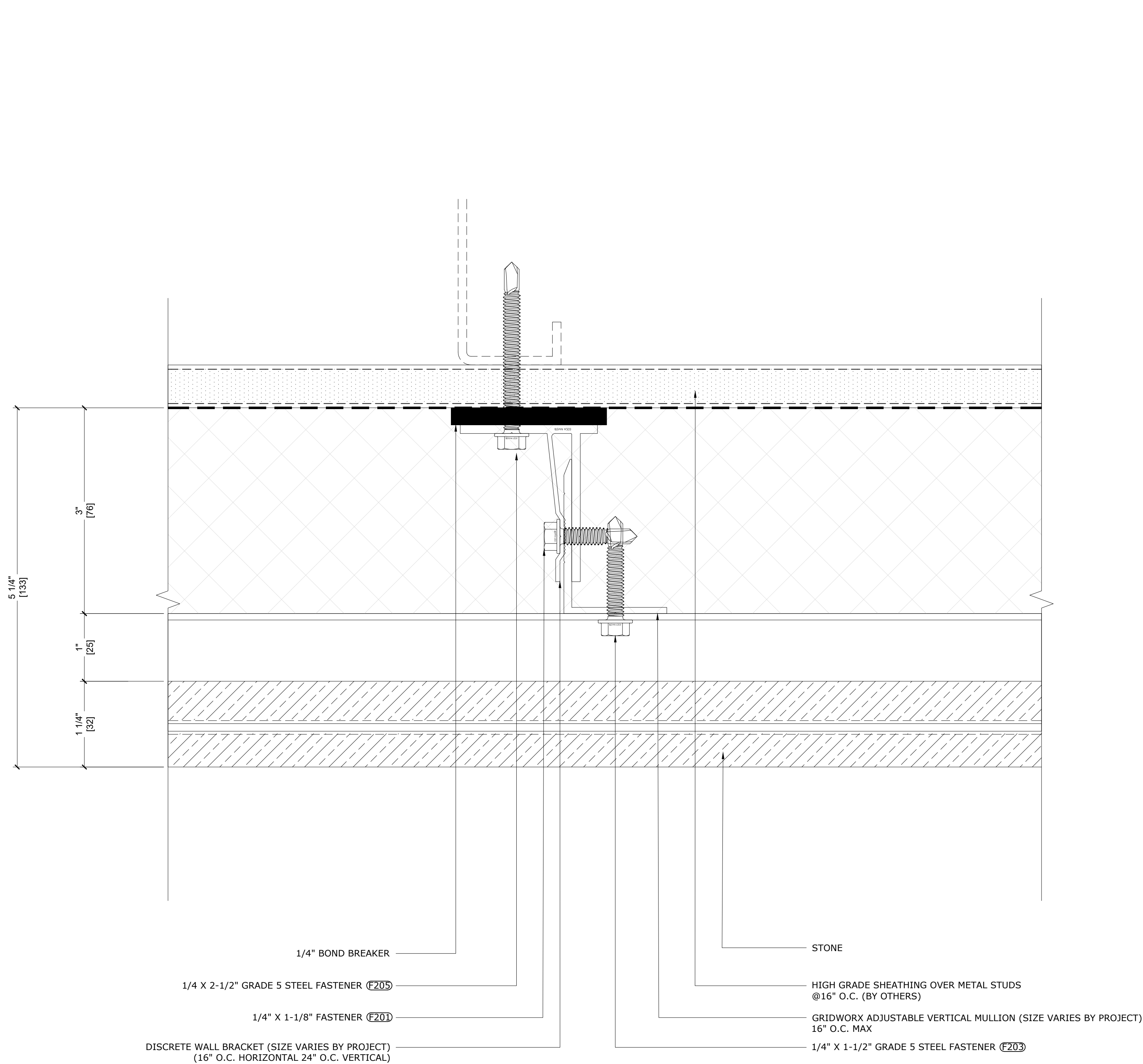
1 PLAN DETAIL - TYPICAL REF: ST2.01
