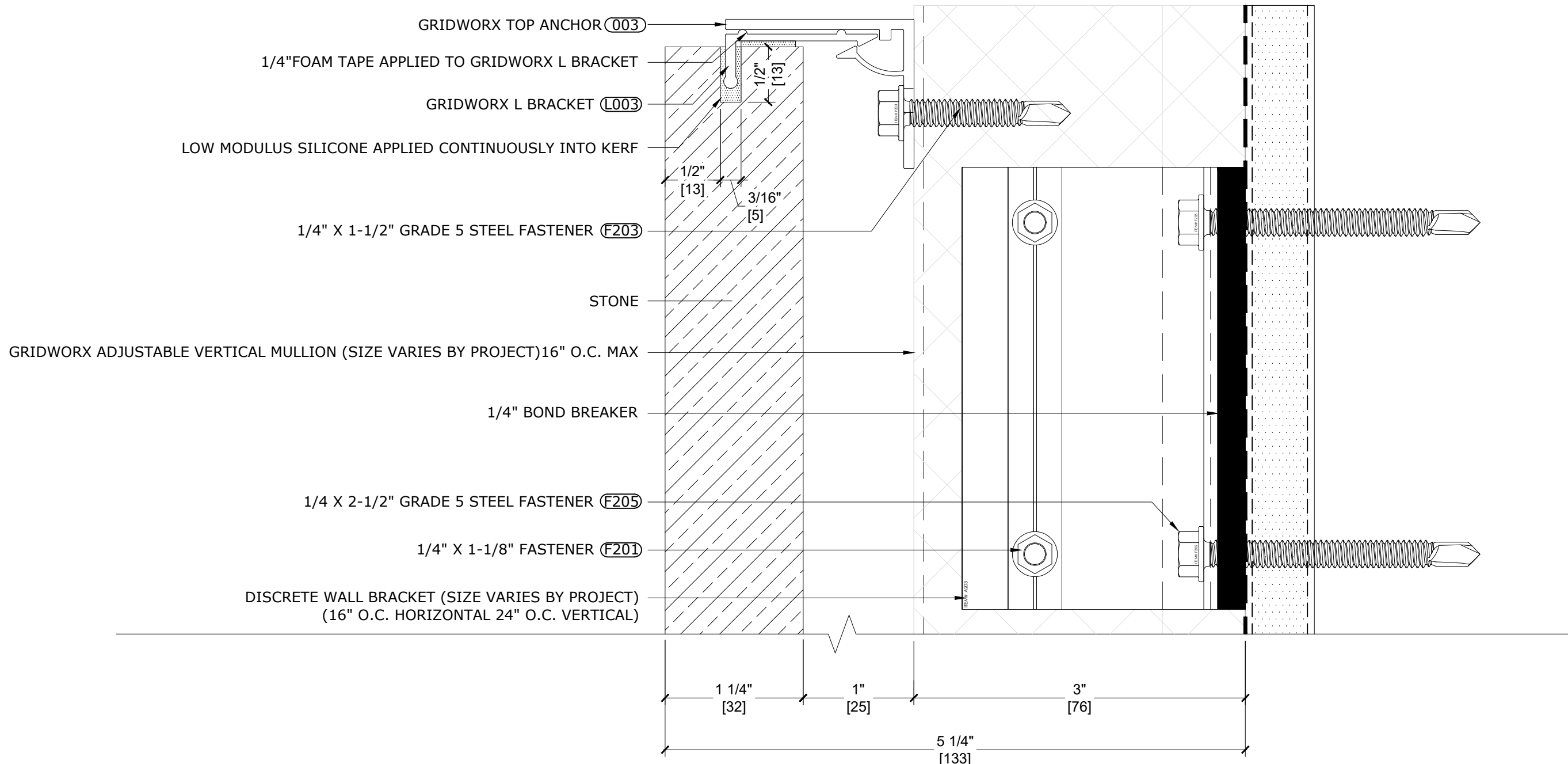
1 SECTION DETAIL - TOP REF: ST2.01
