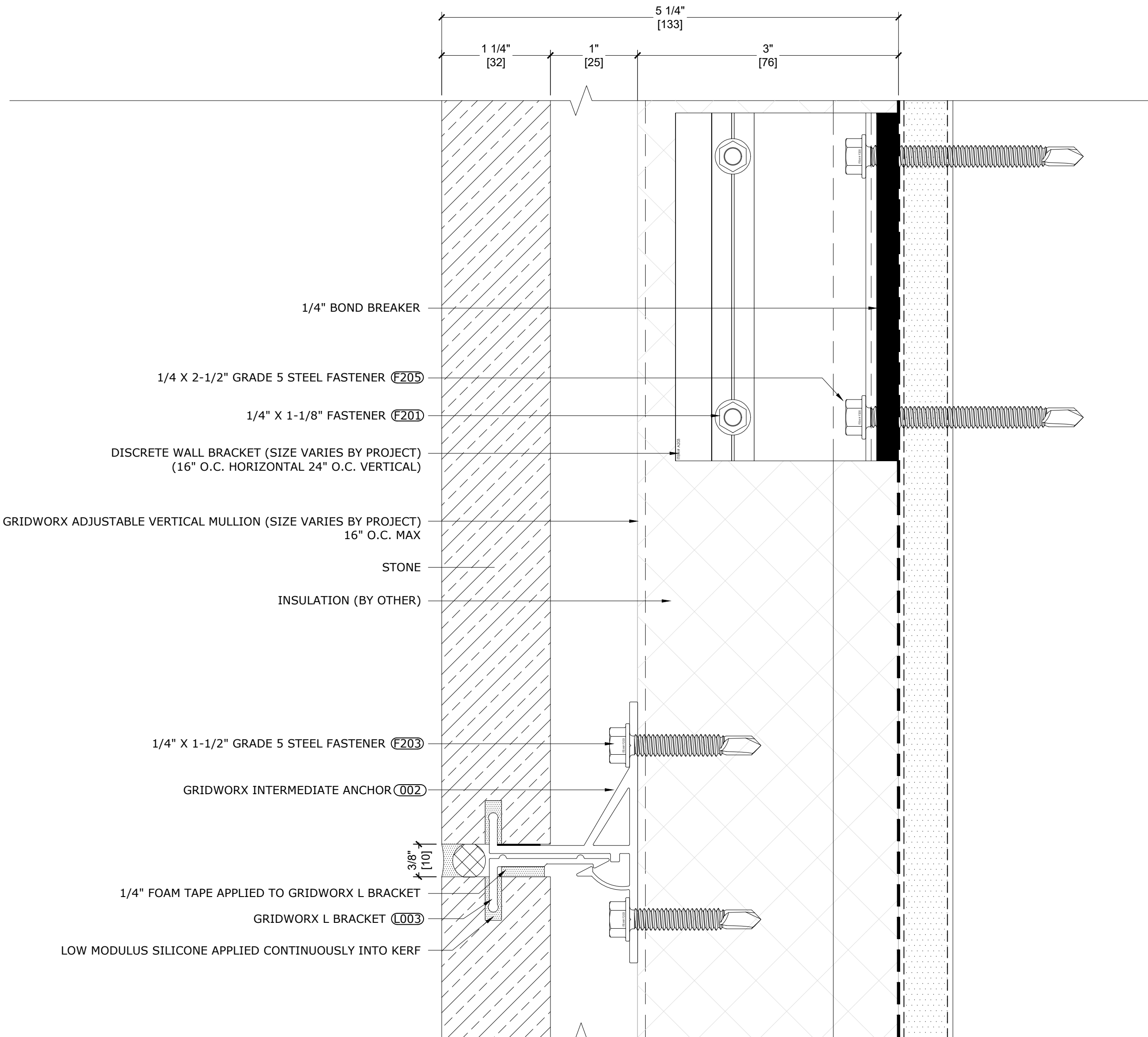
2 SECTION DETAIL - INTERMEDIATE REF: ST2.01
