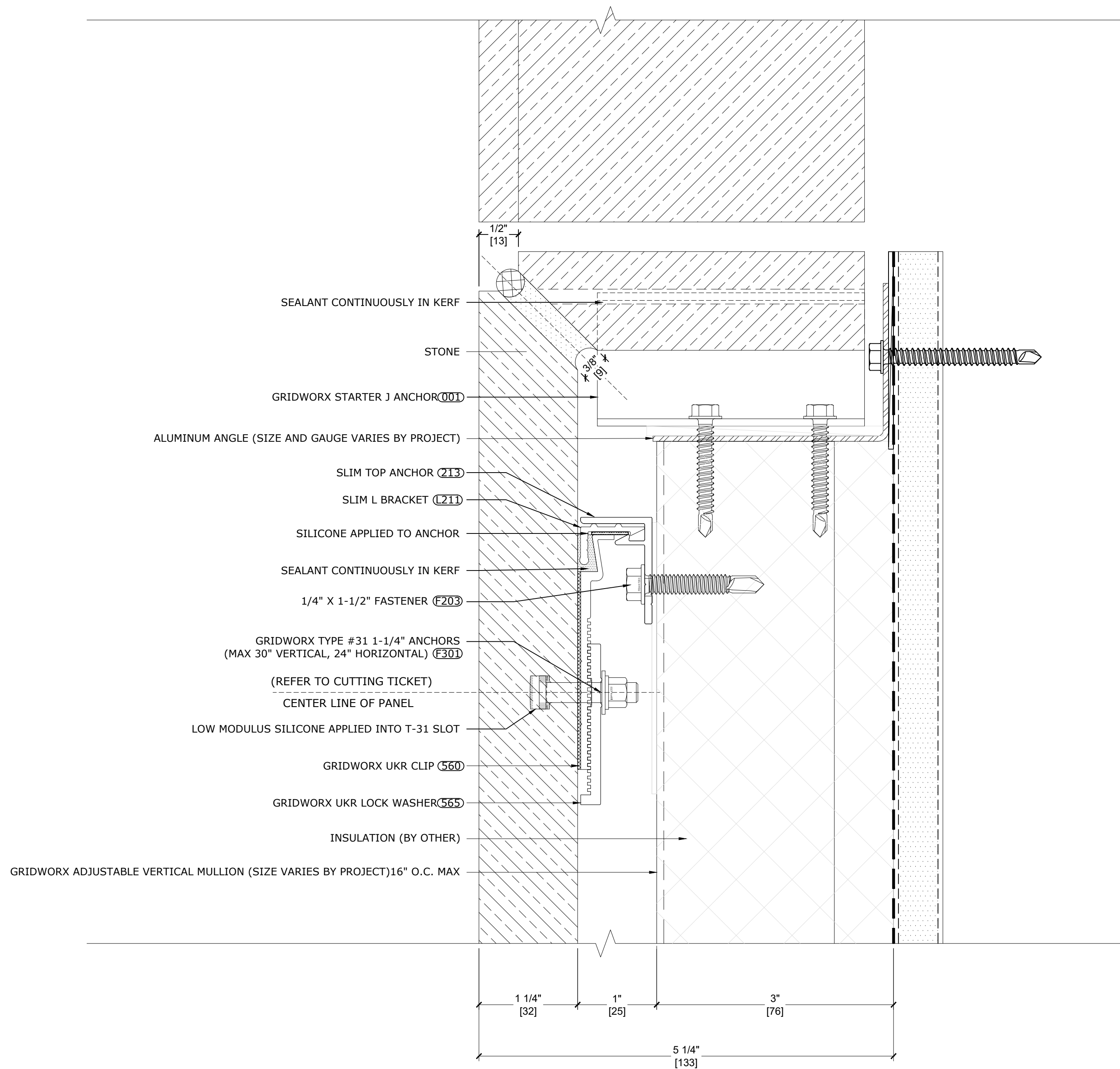
2 SECTION DETAIL - SILL REF: ST2.01
