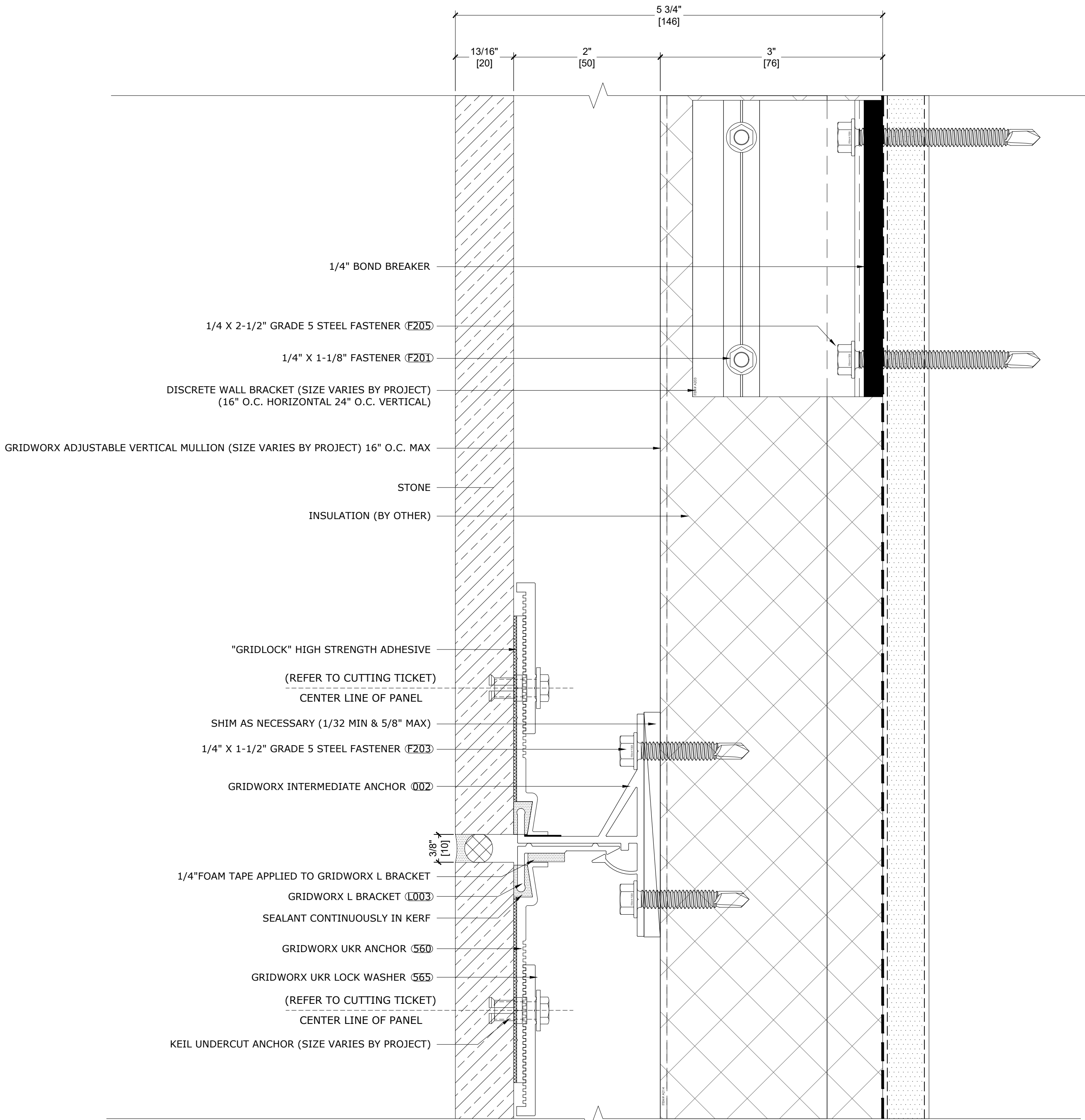
2 SECTION DETAIL - INTERMEDIATE REF: ST2.01
