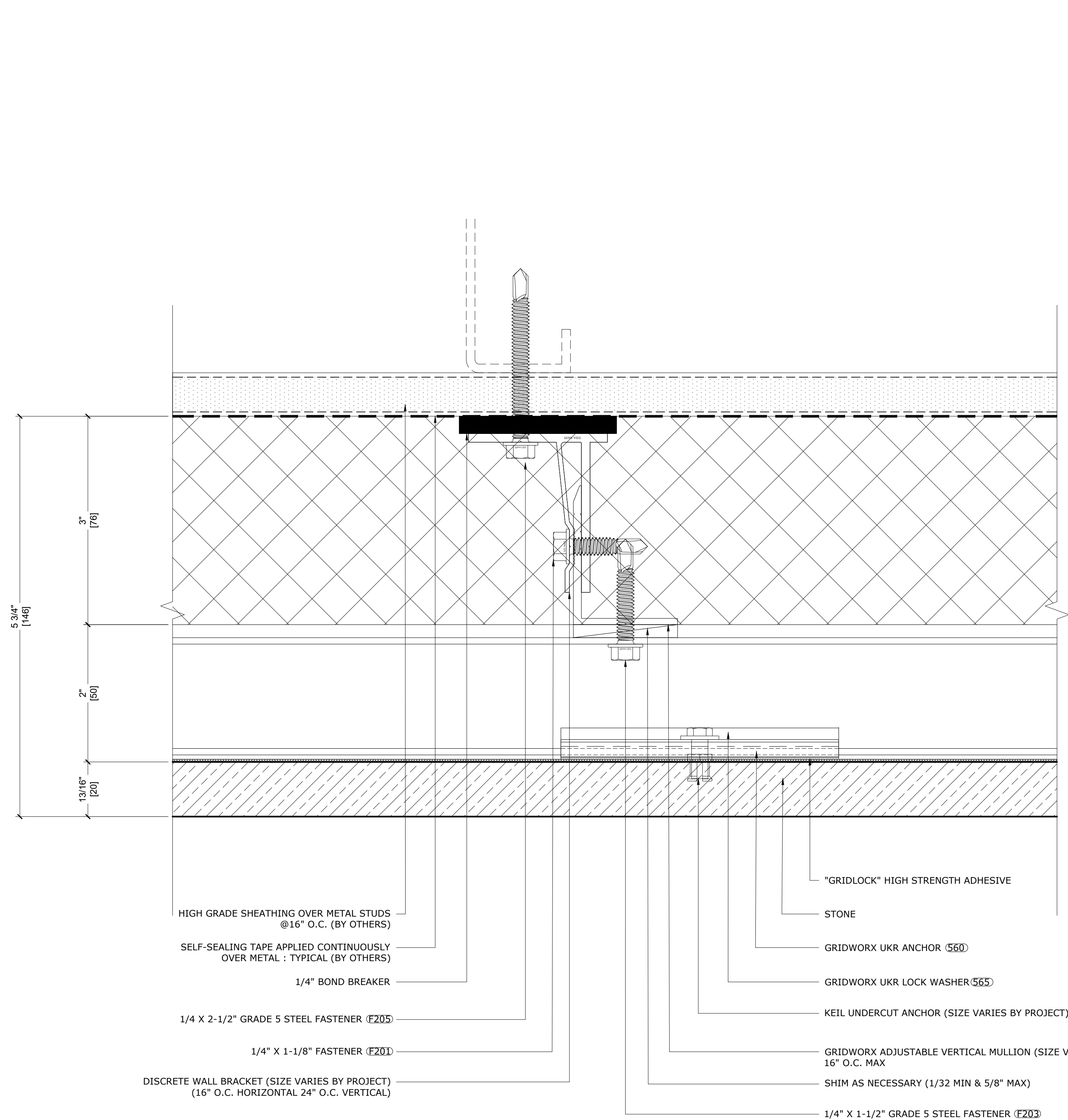
1 PLAN DETAIL - TYPICAL REF: ST2.01
