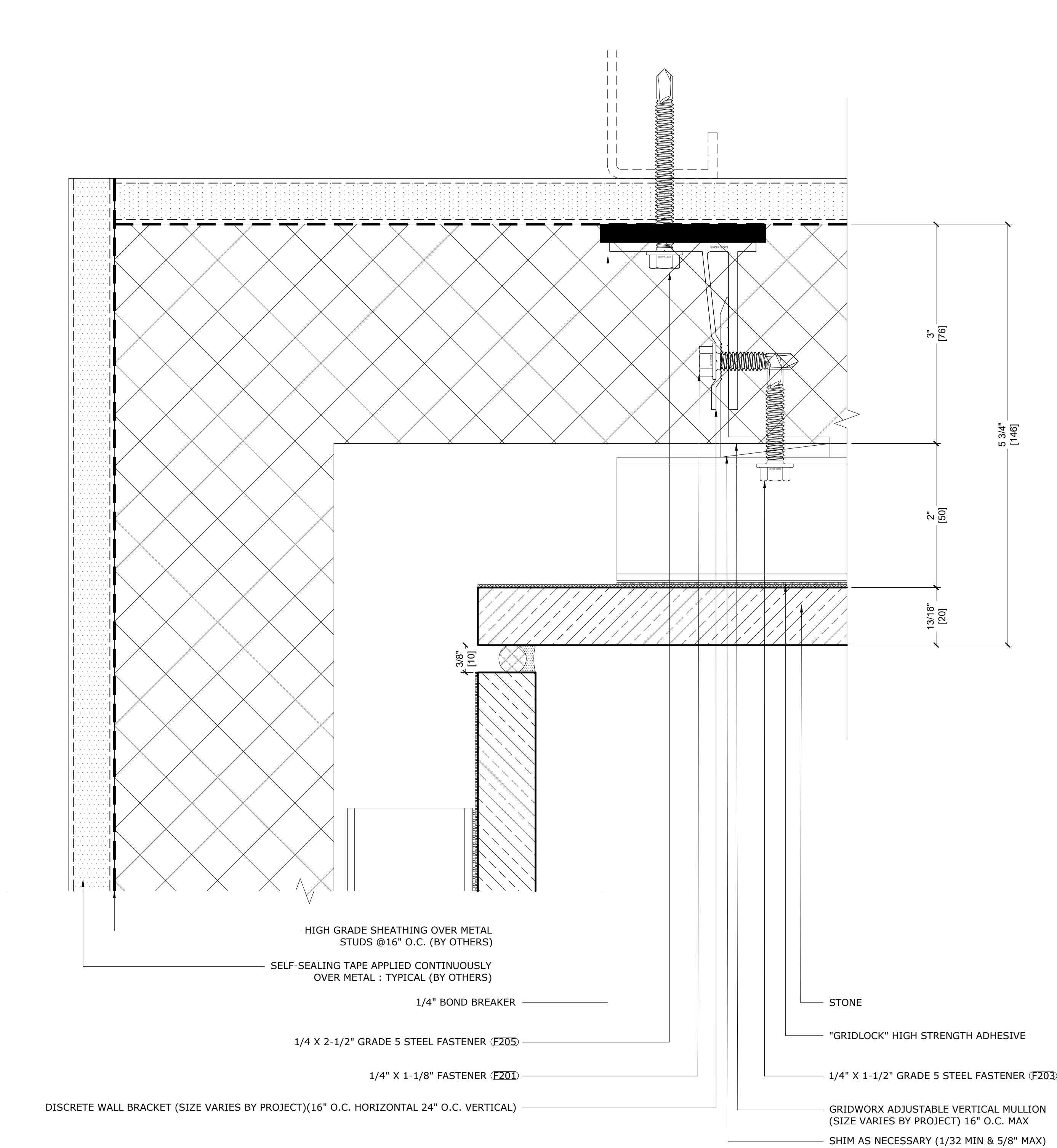
2 PLAN DETAIL - INSIDE CORNER REF: ST2.01
