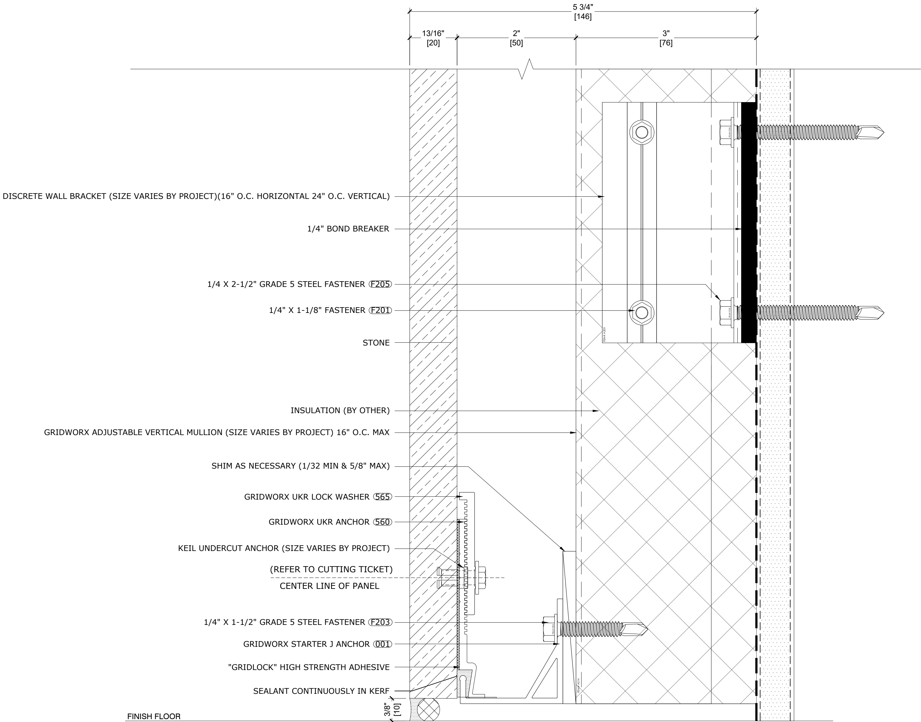
3 SECTION DETAIL - STARTER REF: ST2.01
