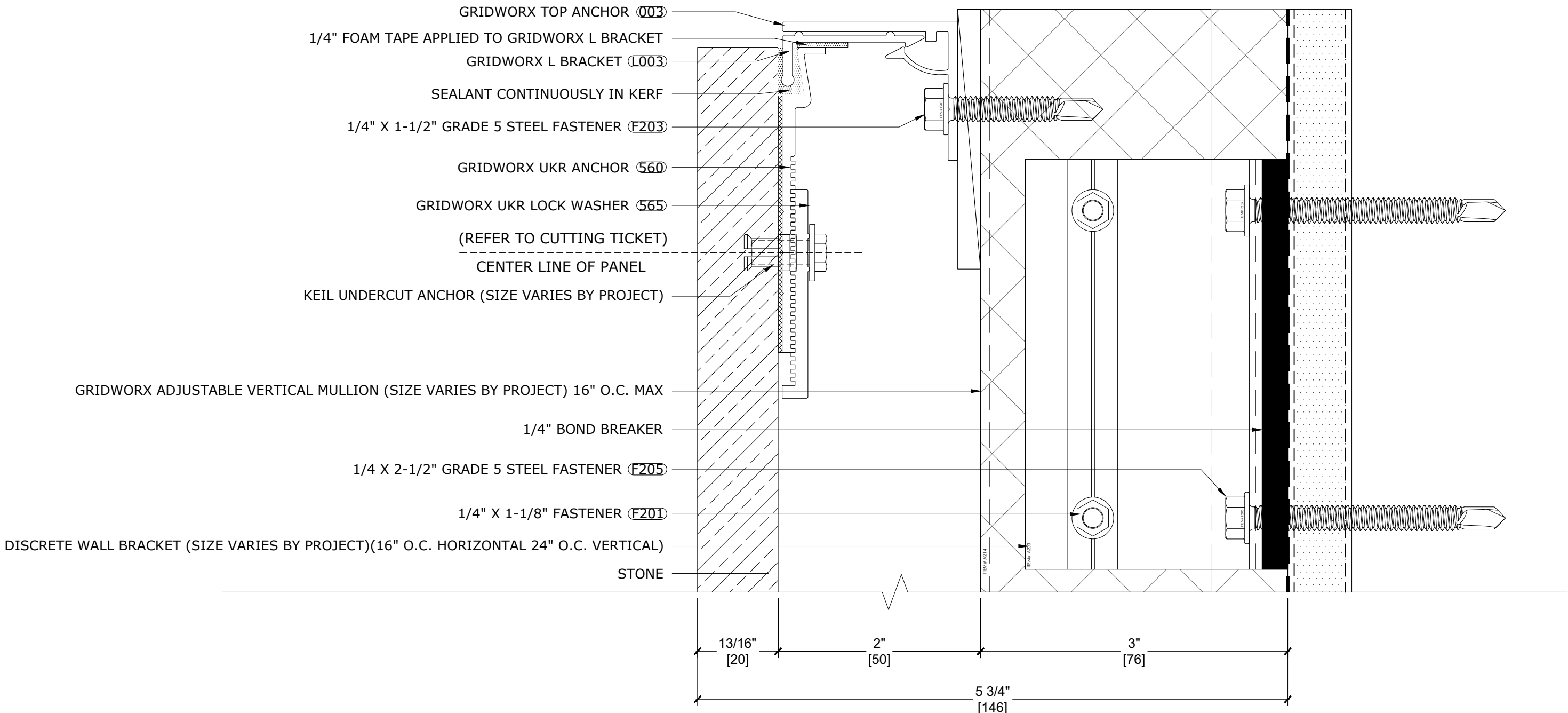
1 SECTION DETAIL - TOP REF: ST2.01
