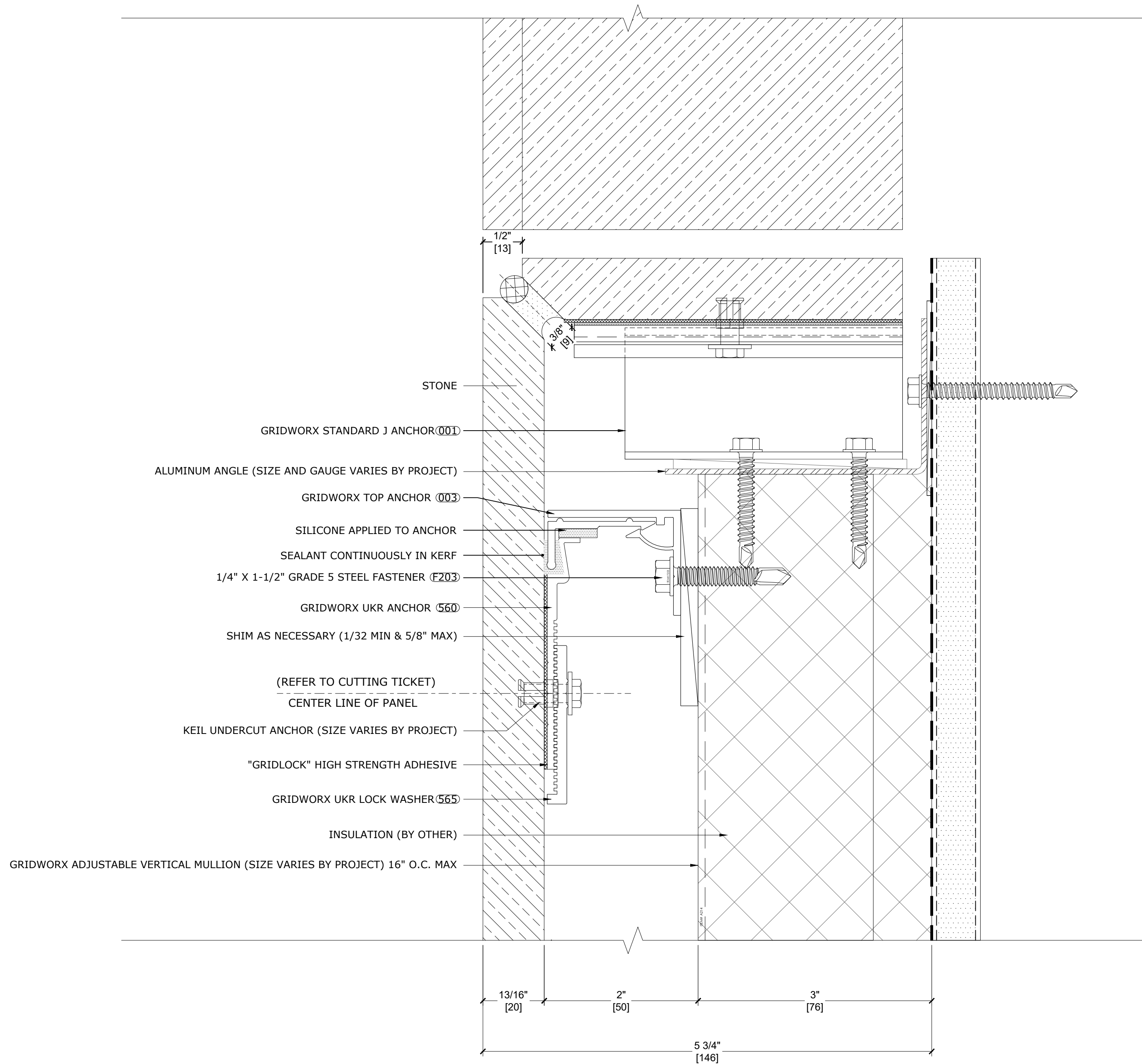
2 SECTION DETAIL - SILL REF: ST2.01
